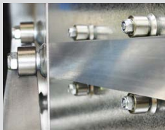
Unique RV Twin Race bearings and stainless steel runners keep your drawers rolling smoothly.
