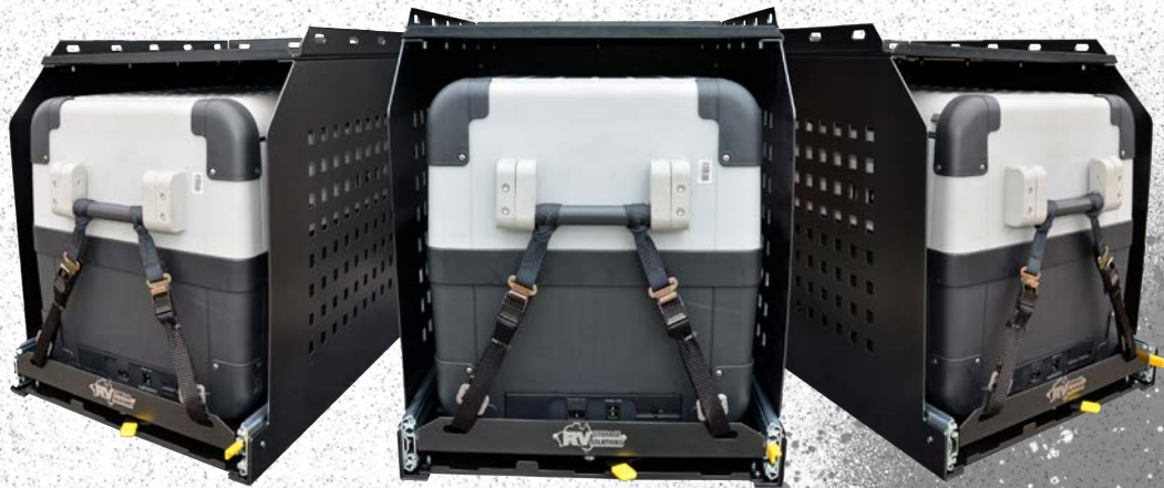
ABOVE: RV Storage Solutions Alloy Fridge Enclosures exclusively designed to fit our RV Heavy Duty Fridge Slides. (Fridge Slide and Straps not included.)
